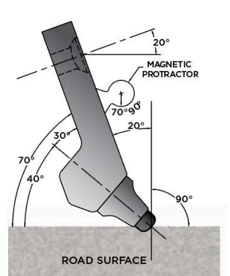
SYSTEM 2000 BOARD AT 20° ANGLE
